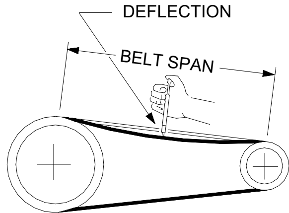
BELT DEFLECTION
